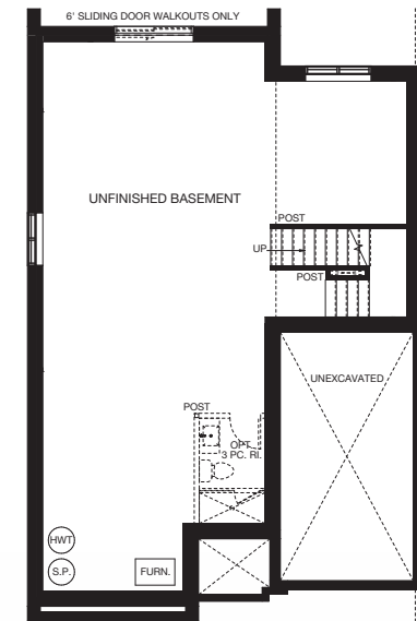
UNFINISHED BASEMENT
