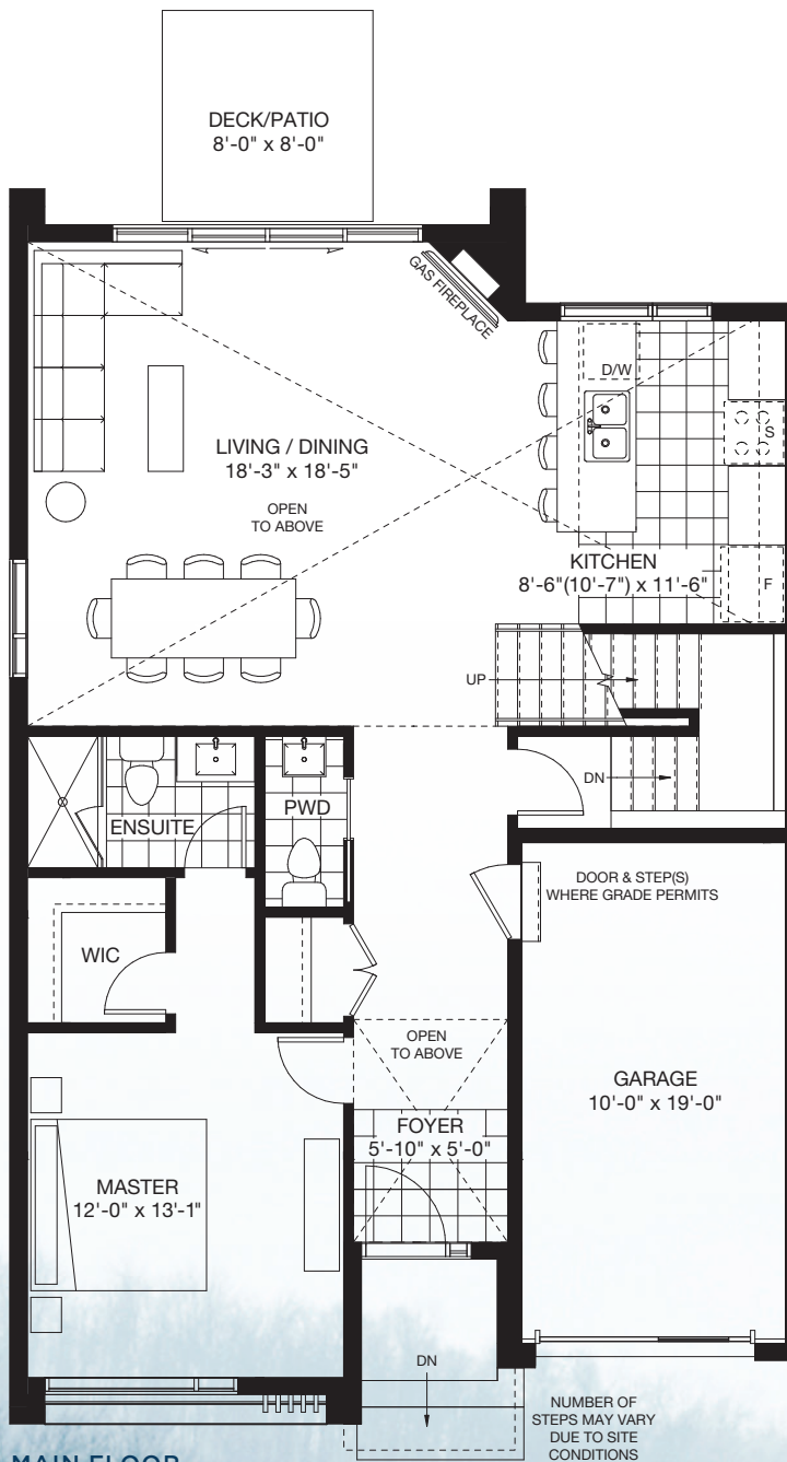
MAIN FLOOR
