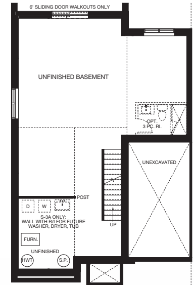
UNFINISHED BASEMENT
