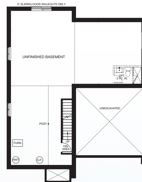
UNFINISHED BASEMENT
