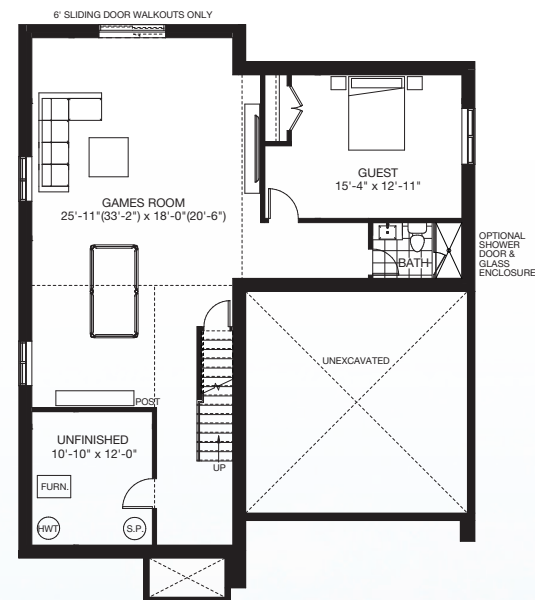
OPT. FINISHED BASEMENT (1,174 SF)
