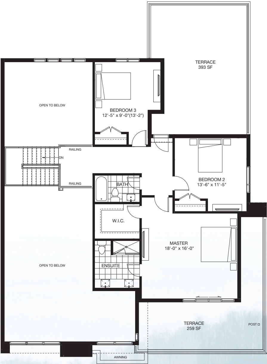
SECOND FLOOR
