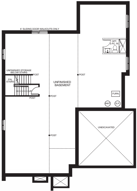
UNFINISHED BASEMENT
