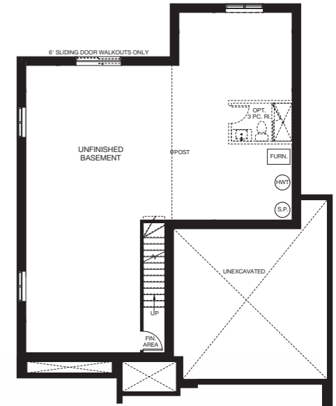
UNFINISHED BASEMENT
