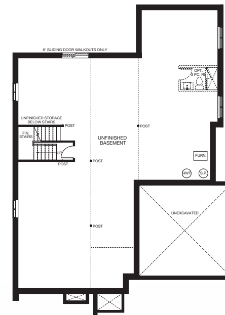
UNFINISHED BASEMENT
