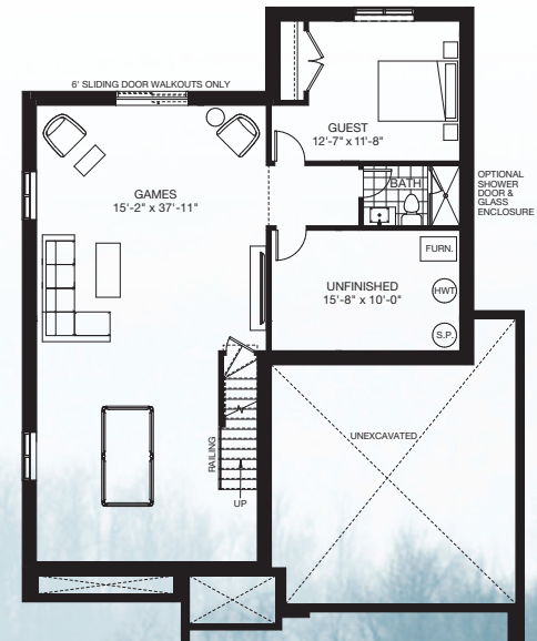
OPT. FINISHED BASEMENT (1,069 SF)
