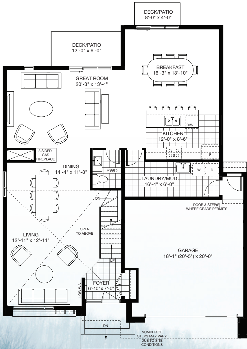
MAIN FLOOR
