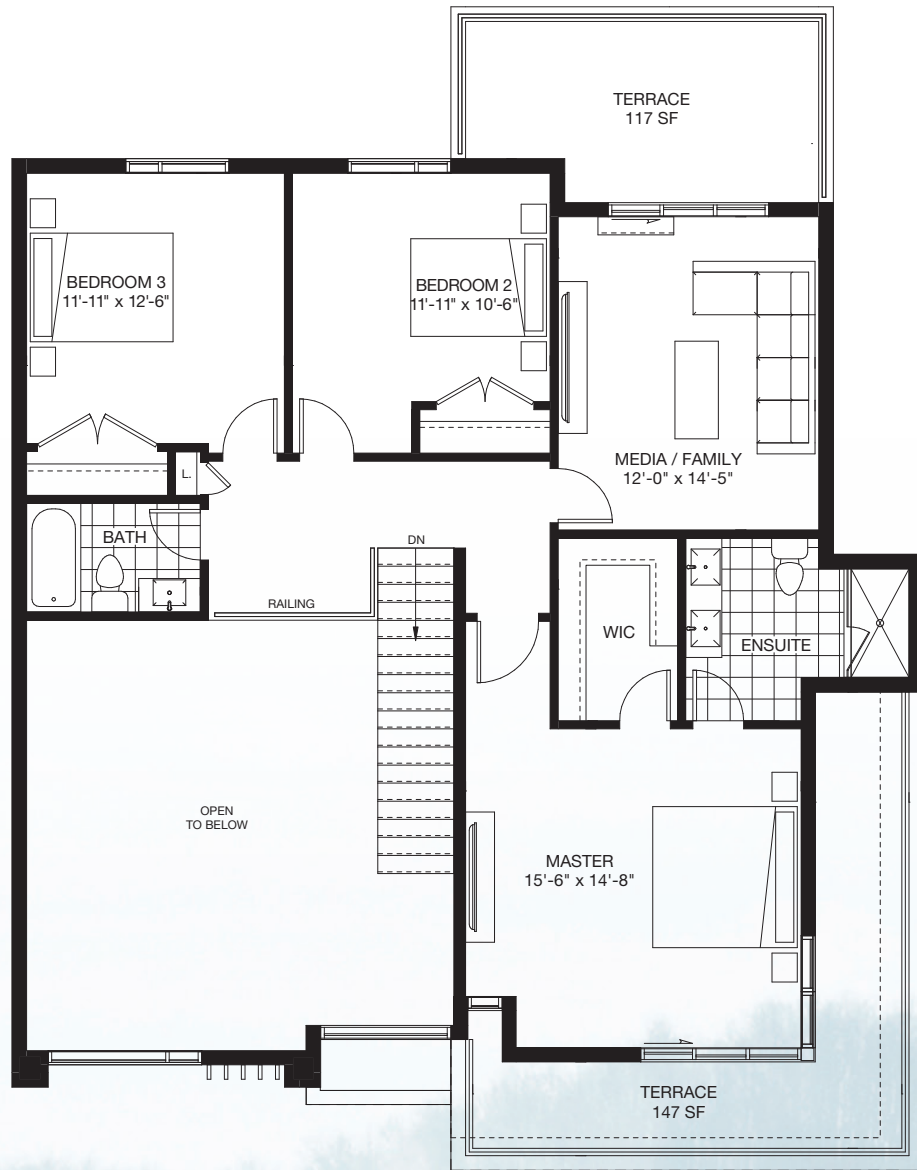
SECOND FLOOR
